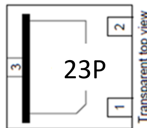
23P = Device Marking Code Bar denotes cathode
